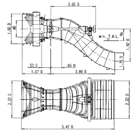
Fig. 2. S-type arrangement
