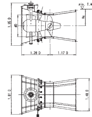
Fig. 1. Tubular arrangement
