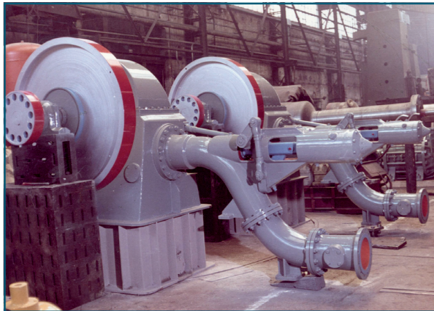
Single jet turbine prior to shipment
