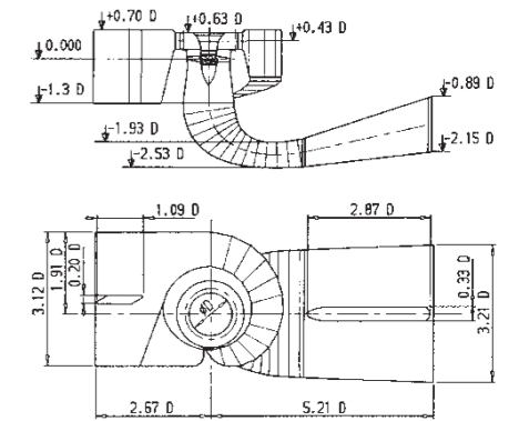
Fig. 4. Concrete soiral case
