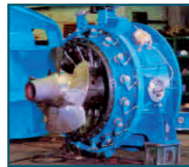
Fig. 2. A tubular Kaplan is prepared for its test run at our premises, Razdan project Armenia
