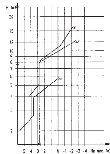
Fig. 7. Admissible turbine settings above tail race level
