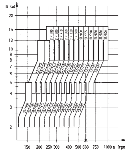
Fig. 6. Applicable speeds
